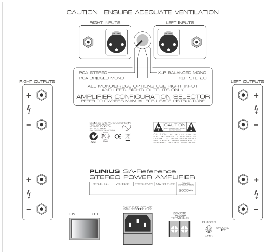
ABOVE: SA-Reference rear panel layout
